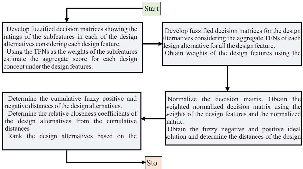
Figure 2: Fuzzy TOPSIS Implementation Process
