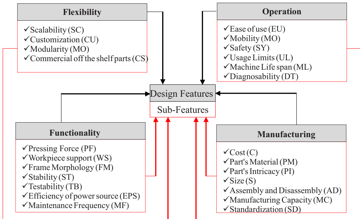
Figure 1: Design Features and Sub-features for Optimal Press Brake Design
